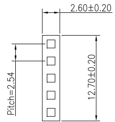
HOUSING
