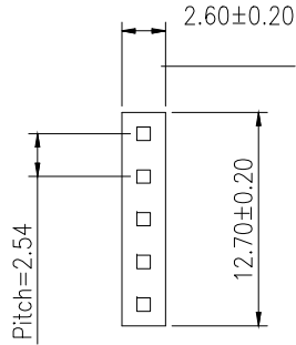
HOUSING
