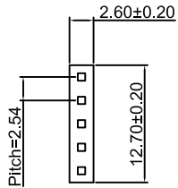
HOUSING
