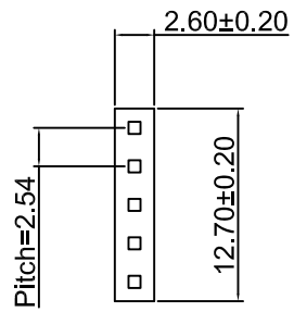
HOUSING
