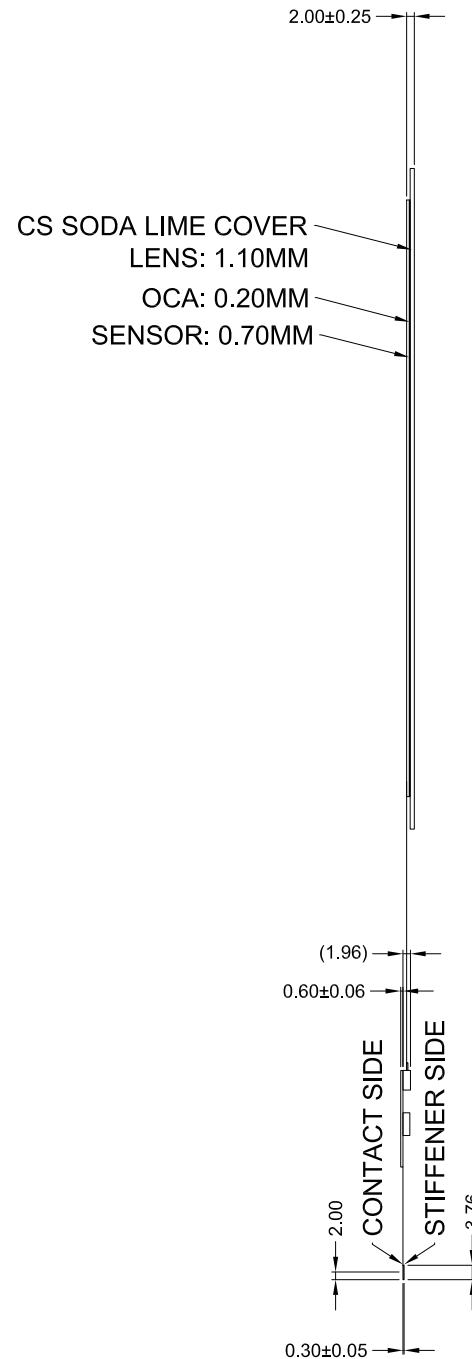
SIDE VIEW
