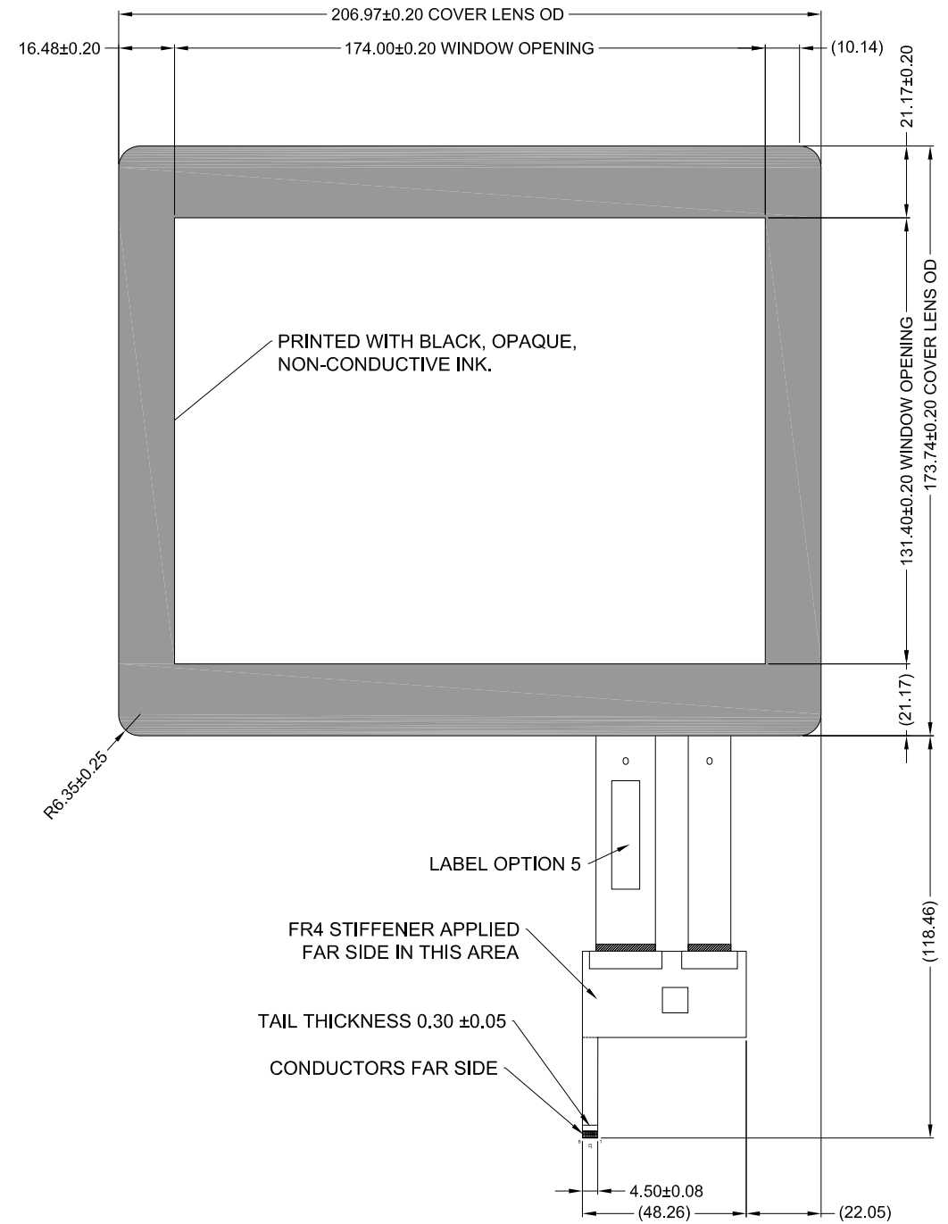
FRONT VIEW
