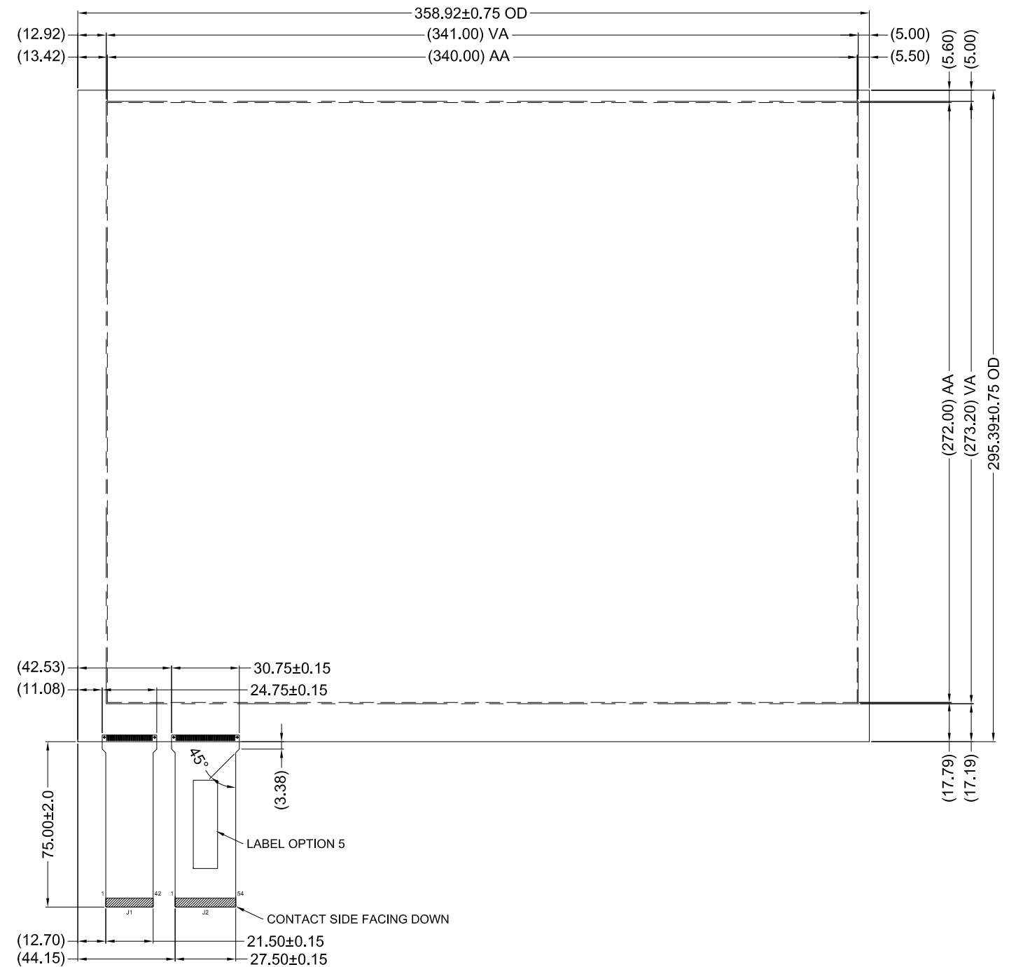
FRONT VIEW
