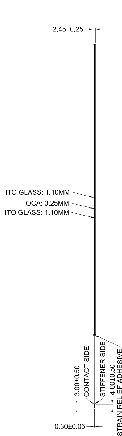
SIDE VIEW
