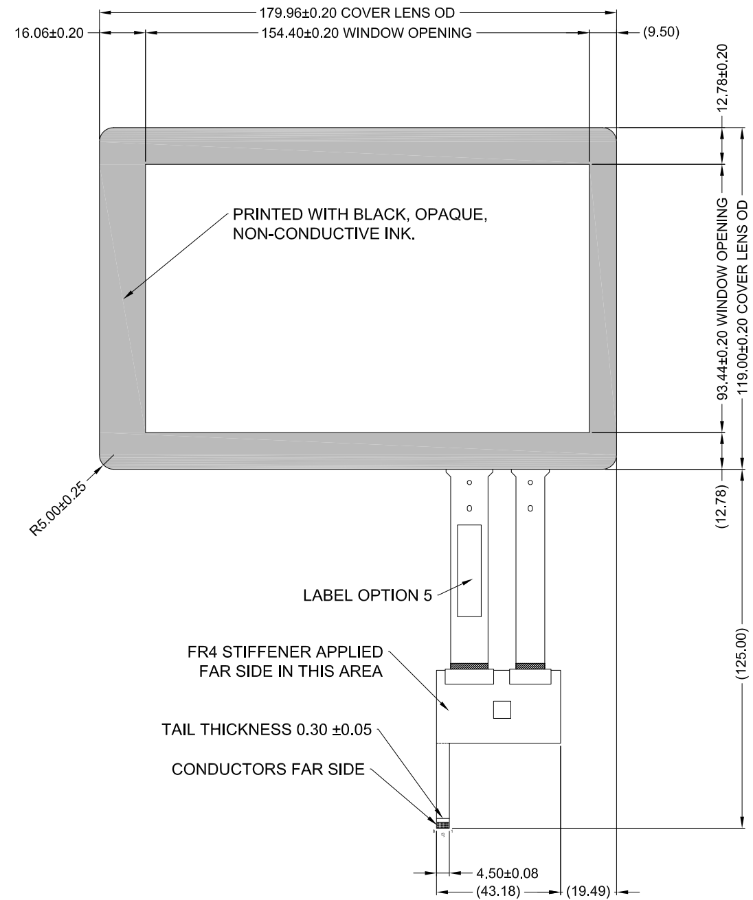
FRONT VIEW
