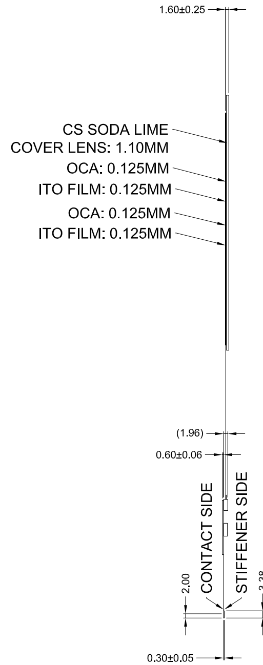
SIDE VIEW
