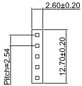
HOUSING
